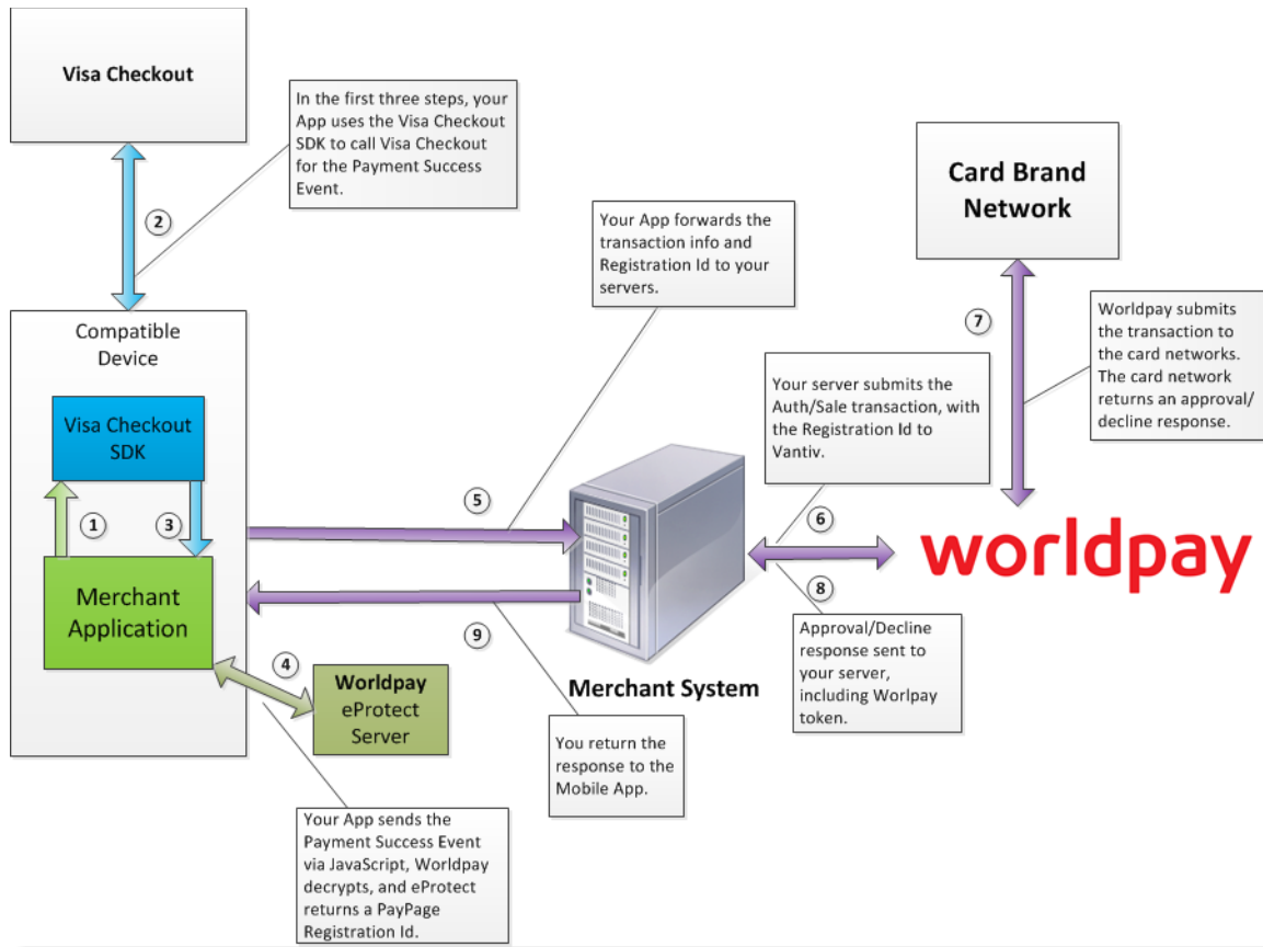
FIGURE 2-4 Data/Transaction Flow using the Worldpay Mobile API for Visa Checkout
