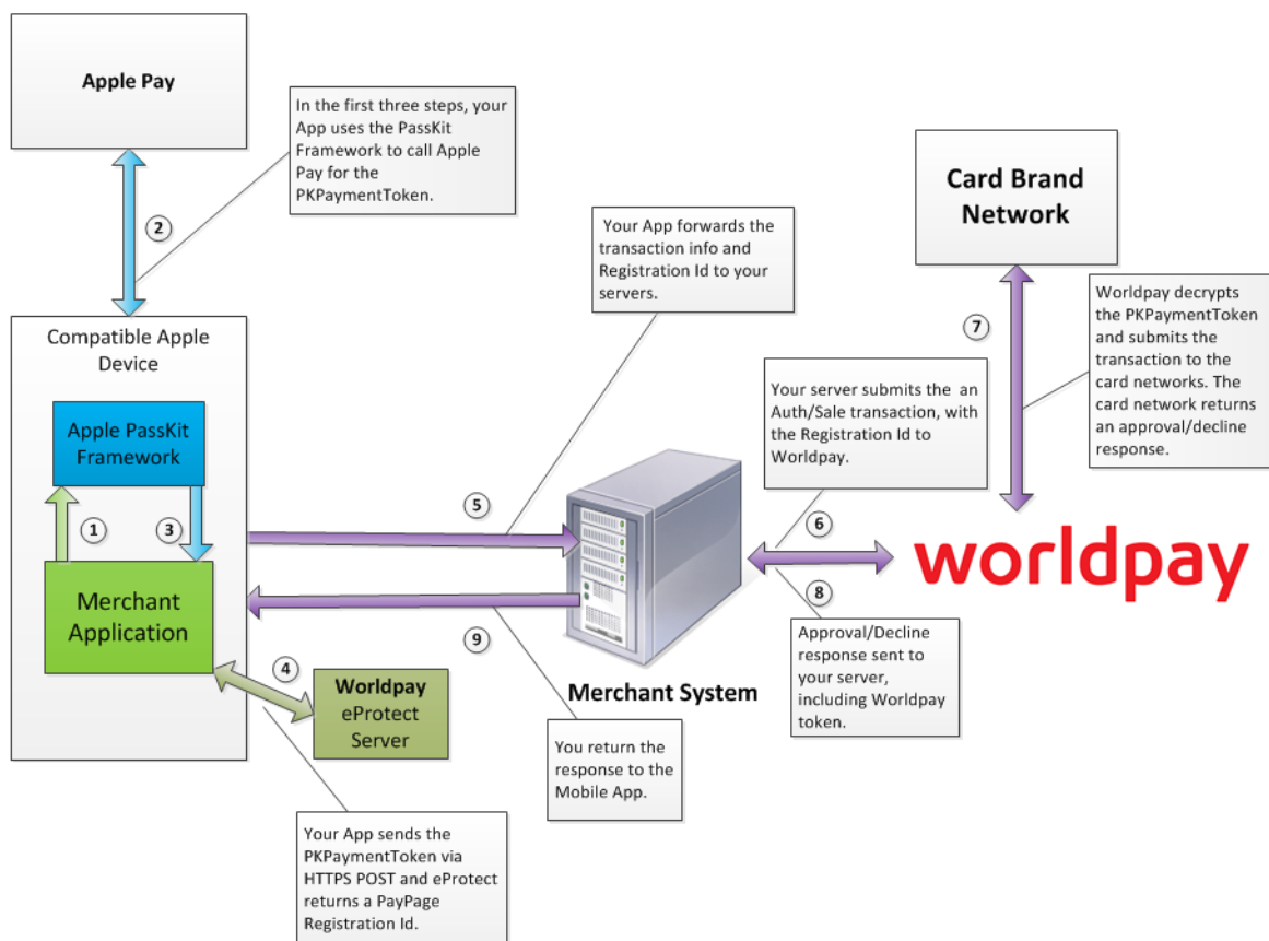
FIGURE 2-3 Data/Transaction Flow using the Worldpay Mobile API for Apple Pay
