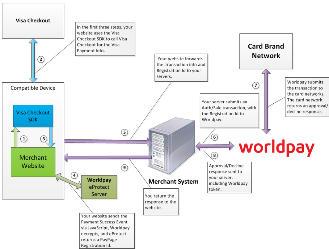
FIGURE 2-2 Data/Transaction Flow - Worldpay Browser JavaScript API for Visa Checkout
