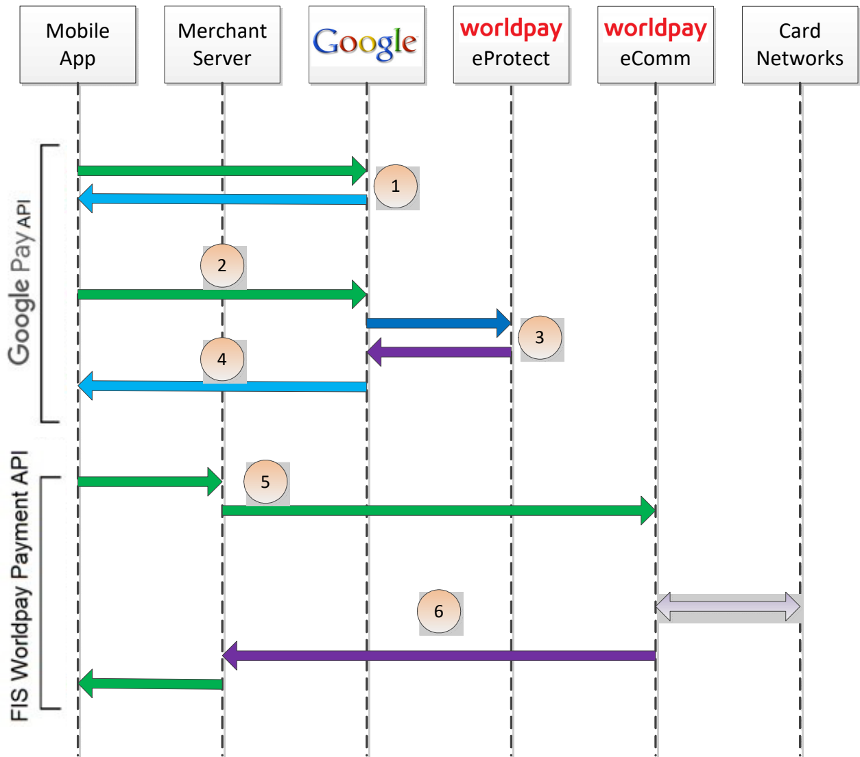
FIGURE 2-5 High Level Message Flow for Google Pay™ using eProtect
